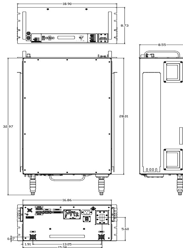
Outline drawing
